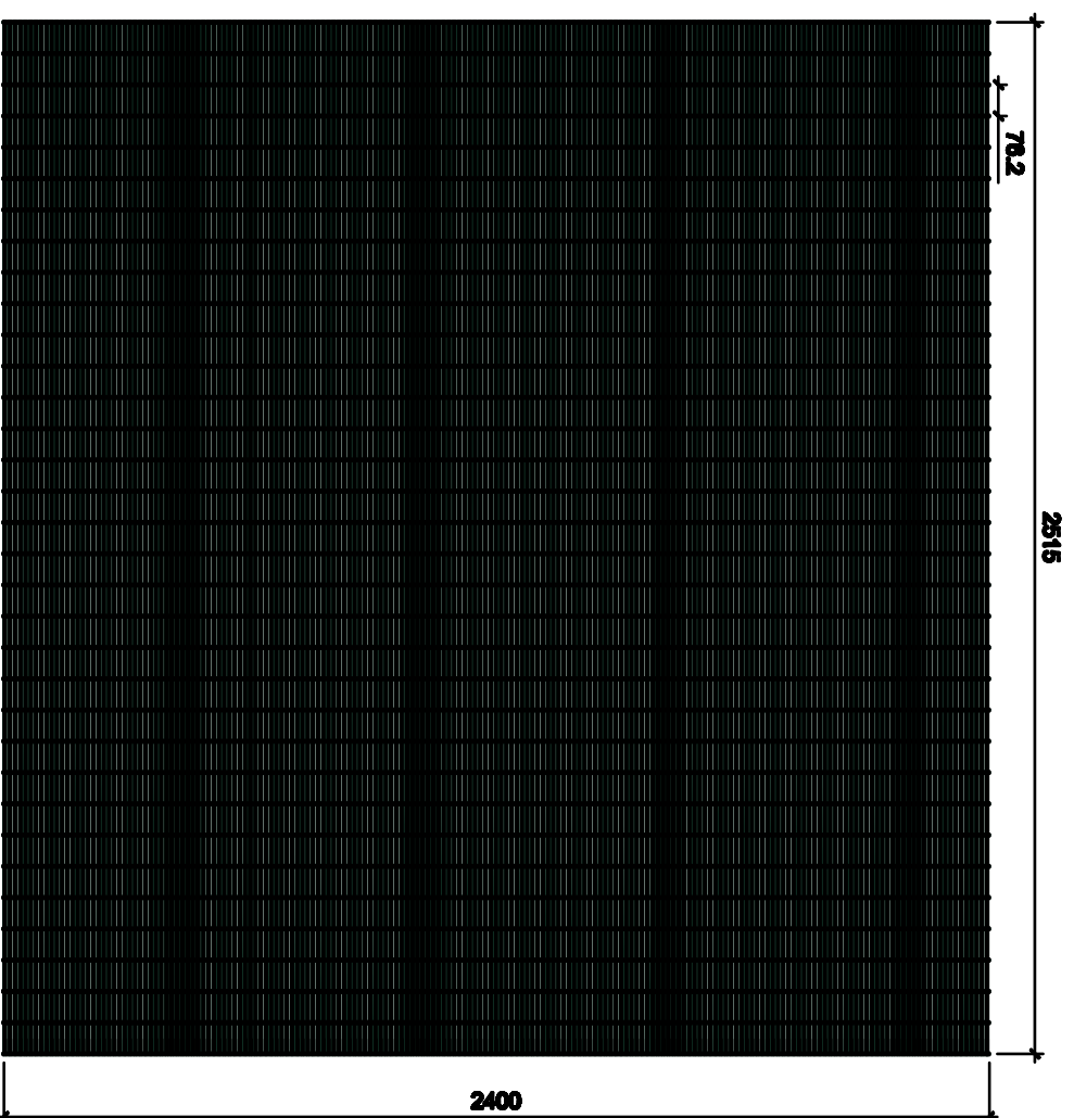
Elevation (2460 high panel) SCALE: 1:2N@A3
