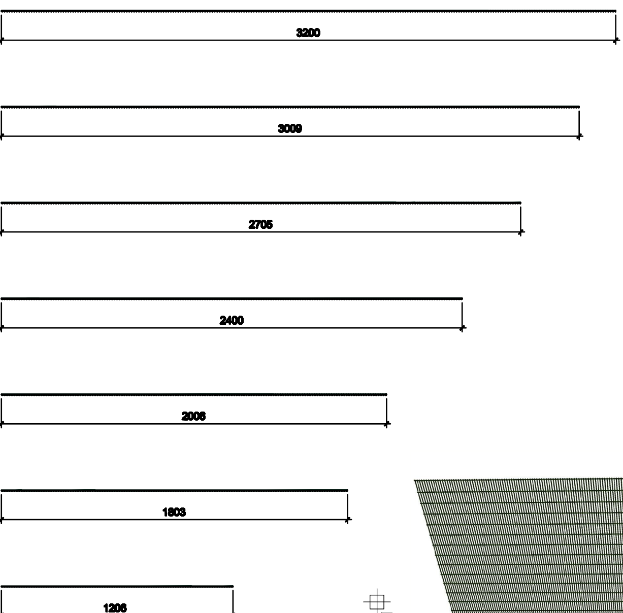
Sections (All heights shown) SCALE: 1:20@A3
