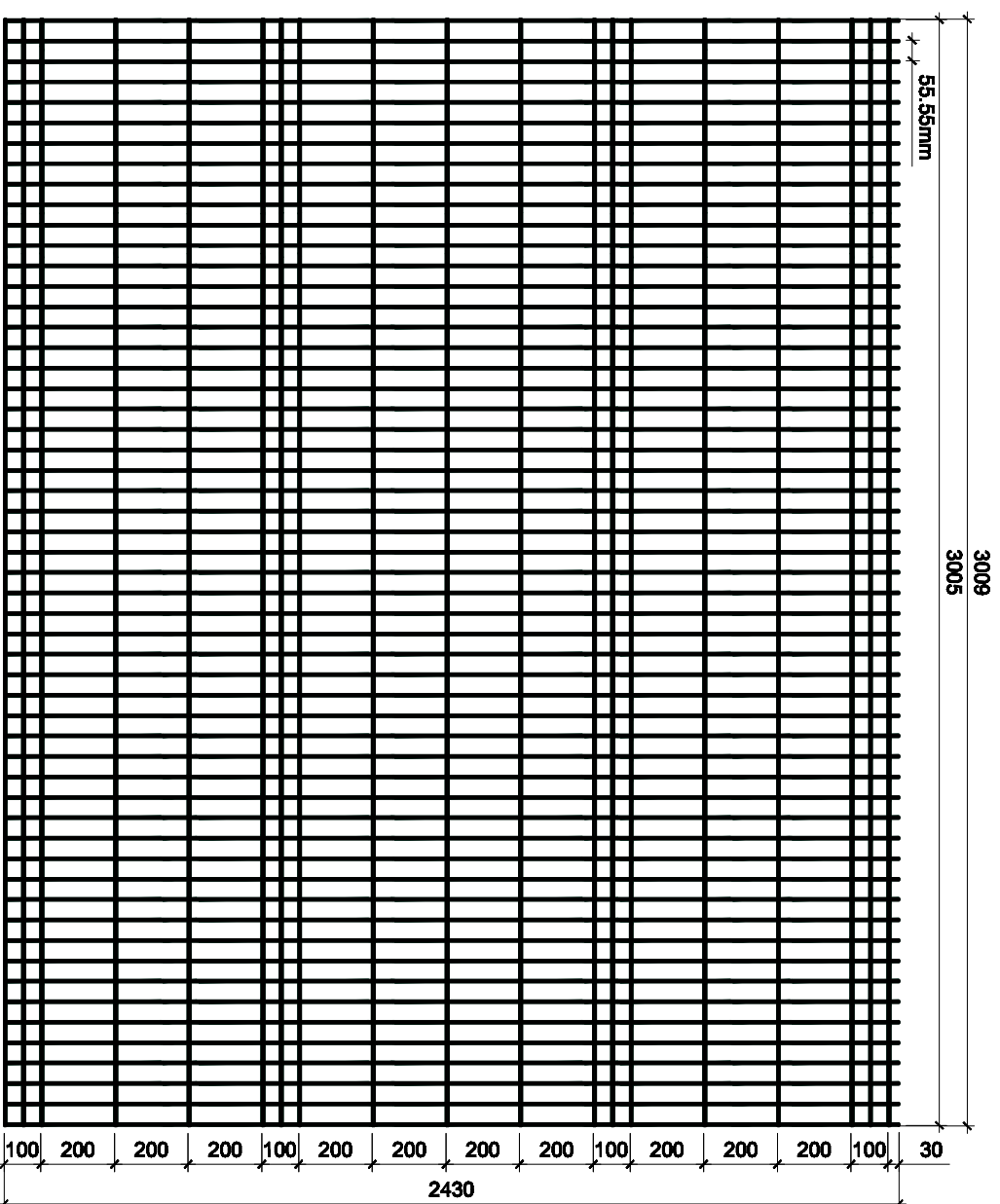
Elevation (2430 high panel) SCALE: 1:20@A3
