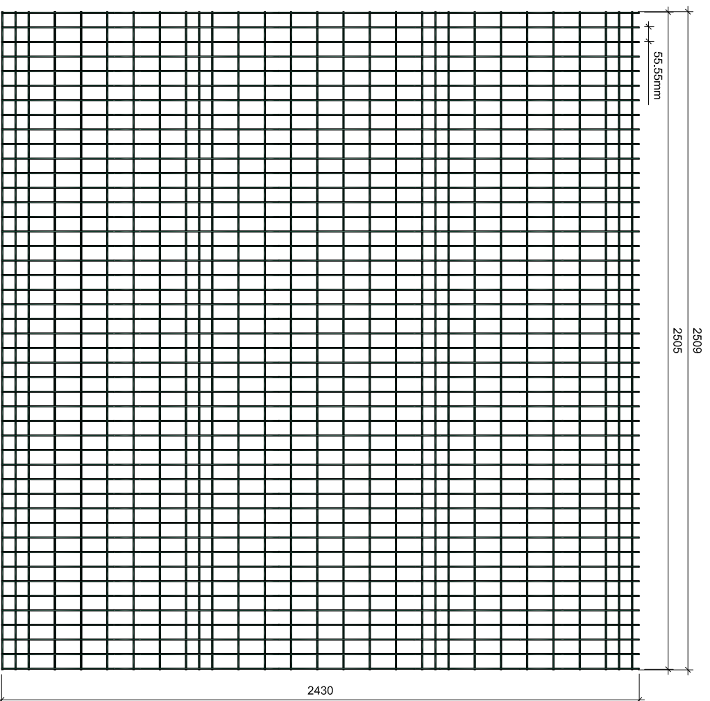
Elevation (2430 high panel) SCALE: 1:20@A3
