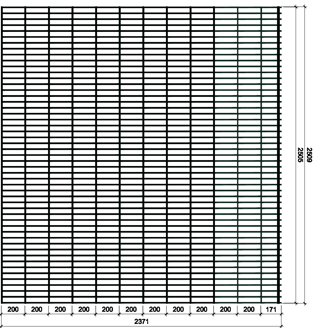
Elevation (2430 high panel) SCALE: 1:20@A3
